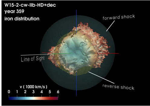
Fig. 1. Isosurface of the distribution of iron at the age of Cas A for one of our simulations (see Orlando et al. 2020b). The opaque isosurface correspond to a value of Fe density which is at 5% of the peak density; the colors give the radial velocity in units of 1000 \text{ km s}^{-1} on the isosurface. The semi-transparent quasi-spherical surfaces indicate the forward (green) and reverse (yellow) shocks. The Earth vantage point lies on the negative y-axis. A navigable 3D graphic of this distribution is available at https://skfb.ly/6TKRK .
