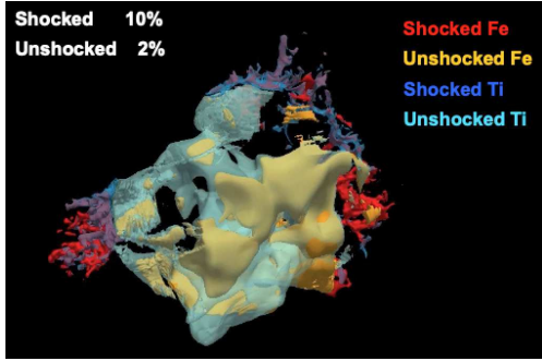
Fig. 2. Isosurfaces of the distribution of iron and titanium at the age of Cas A for one of our simulations (see Orlando et al. 2020b). The irregular isosurfaces correspond to a value of Fe and Ti density at 10% (shocked) or 2% (unshocked) of the maximum density; the colors indicate either shocked or unshocked Fe and Ti as reported in the upper right corner.
