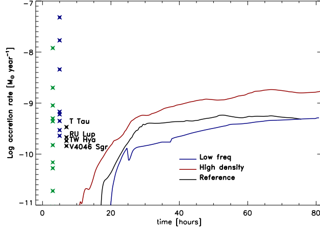
Figure 2: Evolution in time of accretion rate synthesized from simulations. Black line represents the reference case, the red line the high density case and the blue line the low frequency case. The crosses represent the values of mass accretion rate inferred from optical-near UV observations for a sample of low-mass stars and brown dwarfs (green, Herczeg and Hillenbrand 2008), for a sample of solar-mass young accretors (blue, Herczeg and Hillenbrand 2008), and for an X-ray-selected sample of CTTs (black, Curran et al. 2011).
